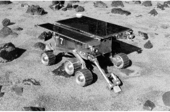
Fig. 1. The Rocky 7 rover.
